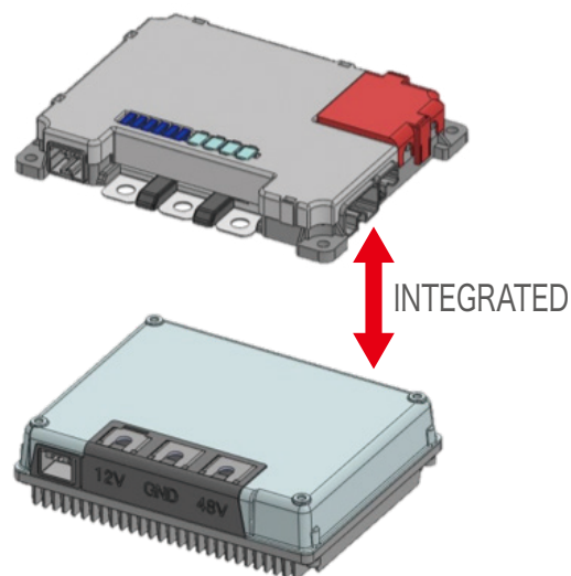
48V-12V DC/DC Converter
